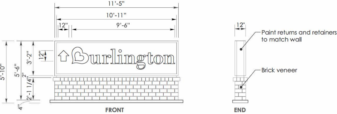
PROPOSED SIGN DIMENSIONS
