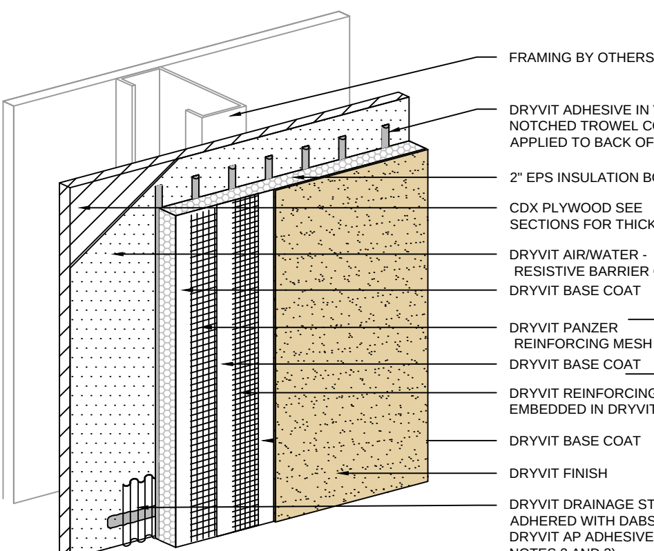
Outsulation® Plus MD System®
