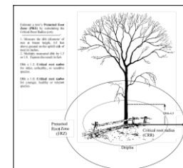
ROOT PROTECTION DURING CONSTRUCTION DETAIL
