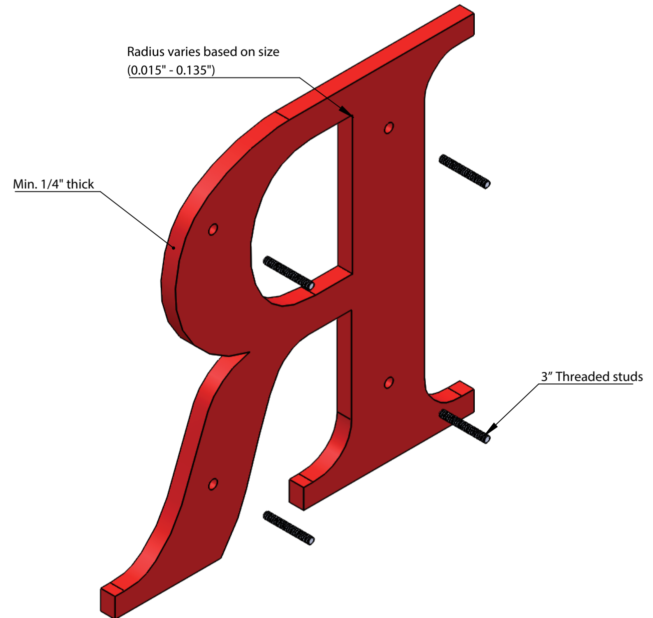
ISOMETRIC BACK VIEW II SCALE 1:3
