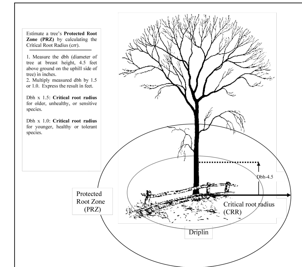
ROOT PROTECTION DURING CONSTRUCTION DETAIL SCALE - N.T.S.
