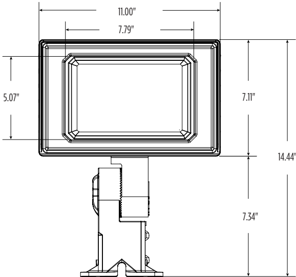
Slip Fitter/Trunnion (SF) Mounting
