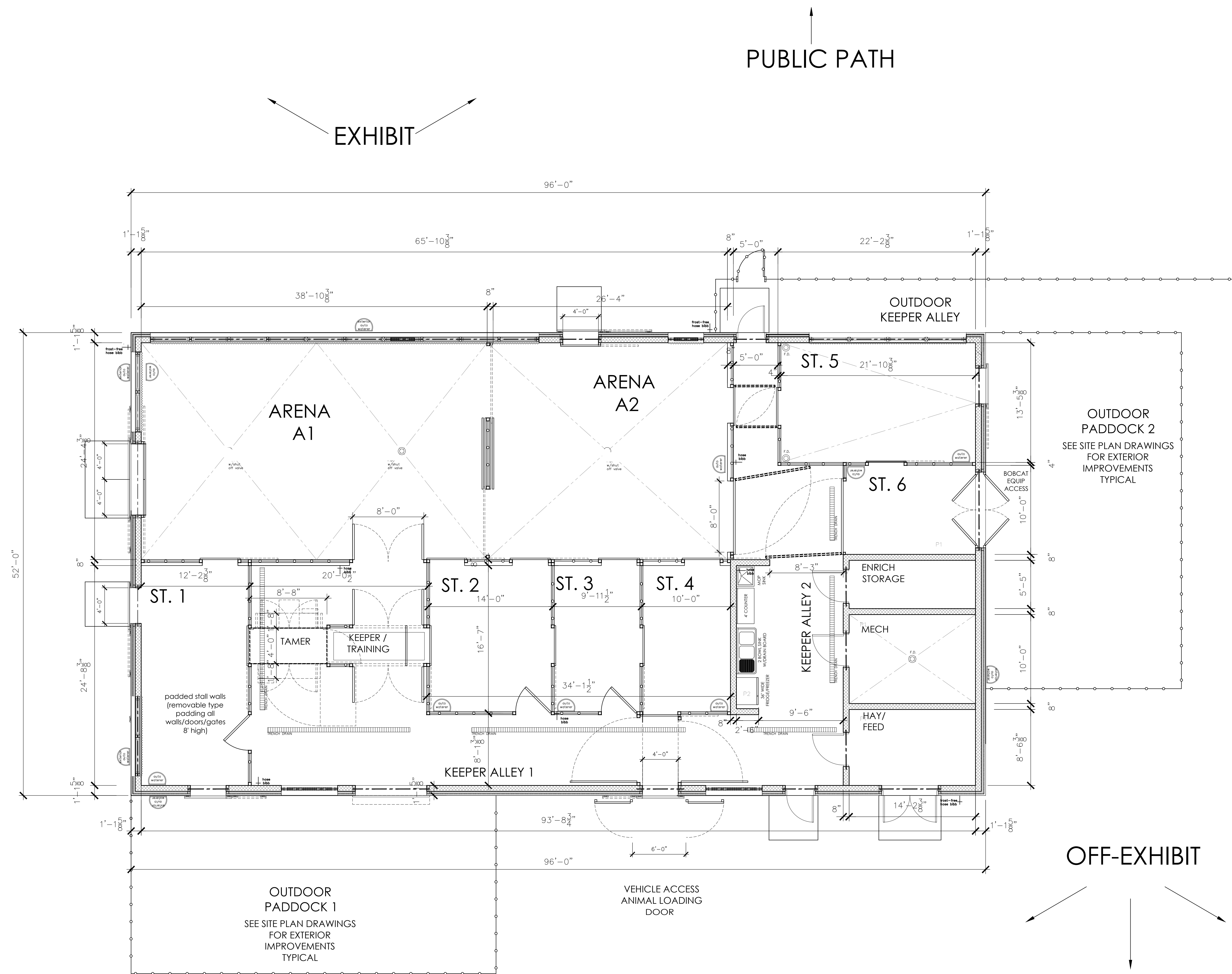
1 GROUND FLOOR PLAN A-1.1 SCALE: 3/16" = 1'-0"
