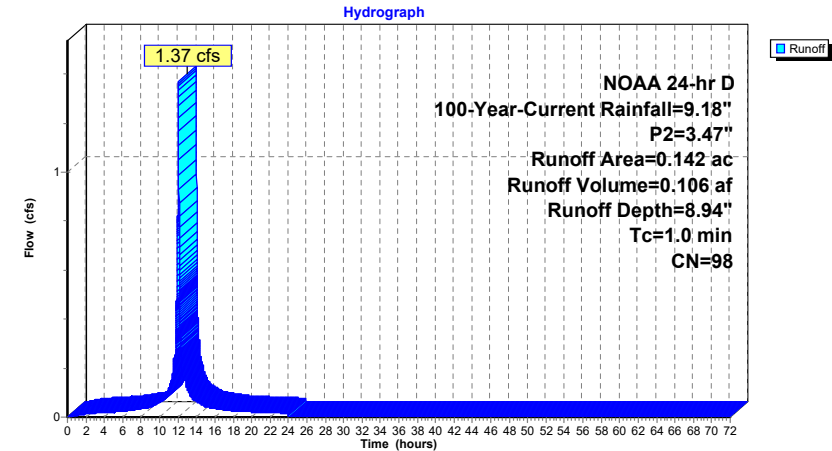
Subcatchment 7S: Proposed Roof
