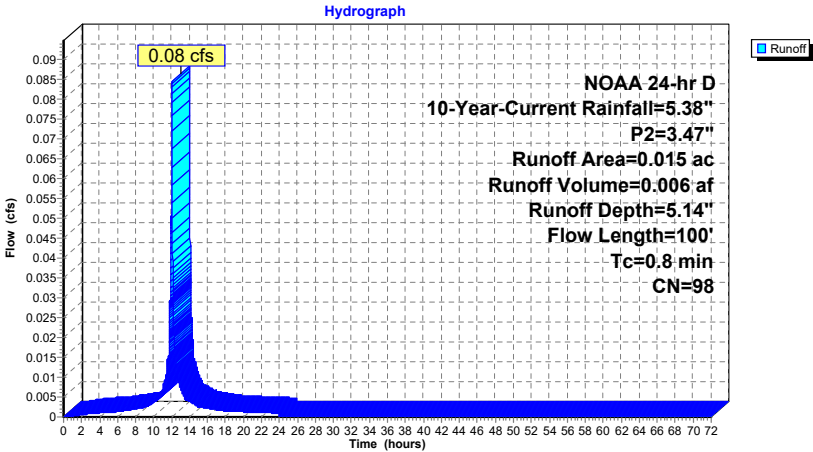
Subcatchment 3S: EDA #2 - Impervious
