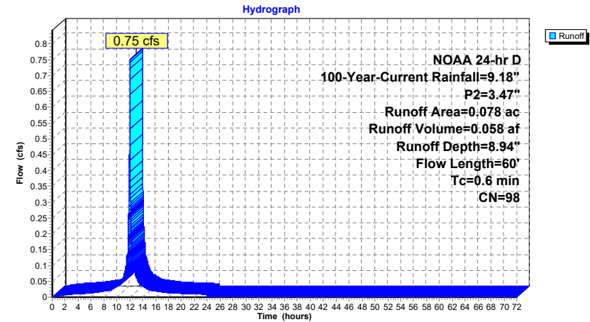
Subcatchment 8S: PDA #1 - Impervious to Bio
