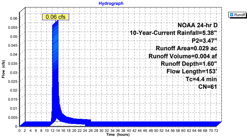
Subcatchment 4S: EDA #2 - Pervious
