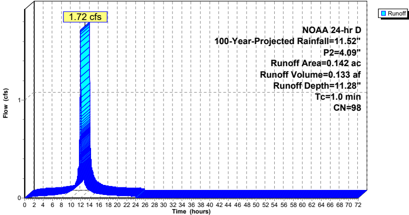
Subcatchment 7S: Proposed Roof
