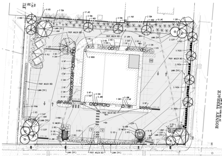
LANDSCAPE PLAN (submitted 03.09.26)
