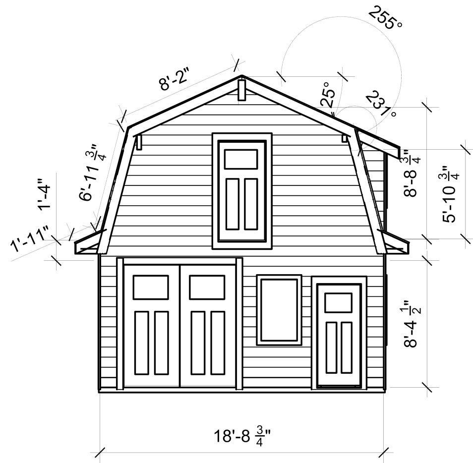
Street Elevation
