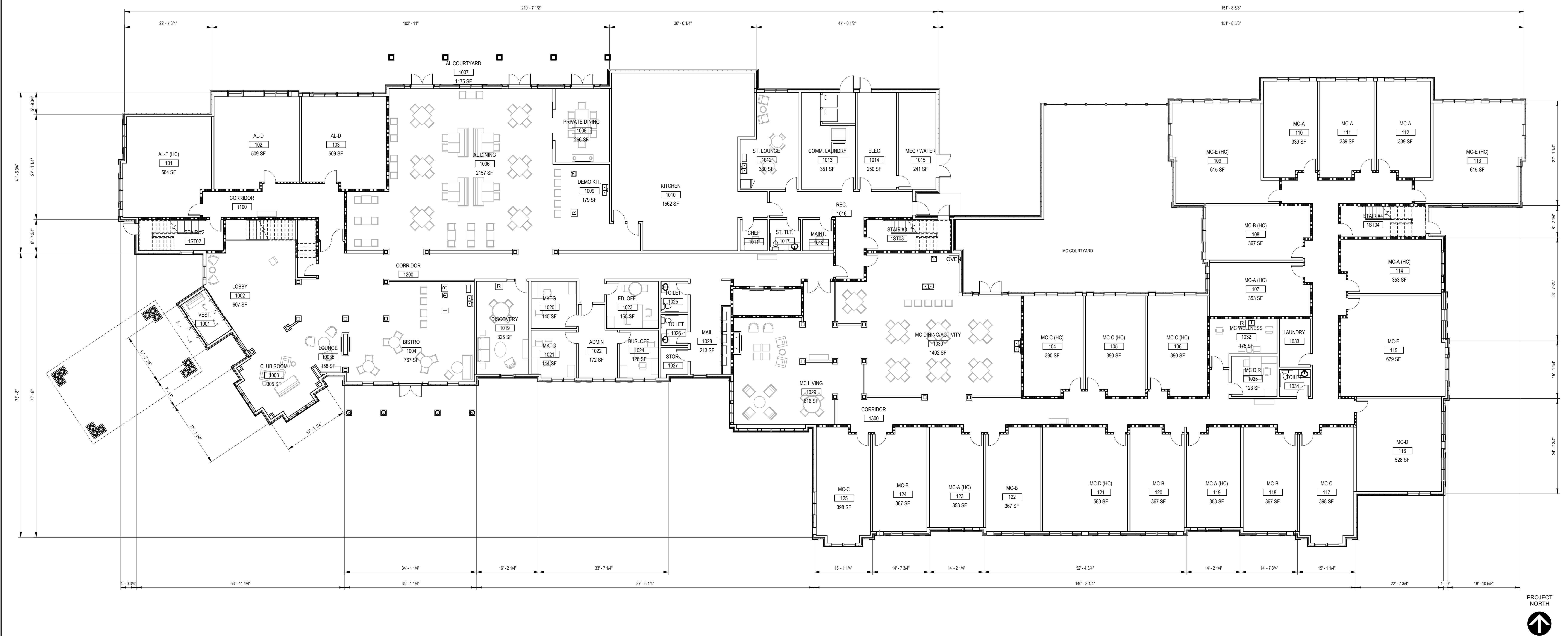
FIRST FLOOR PLAN
