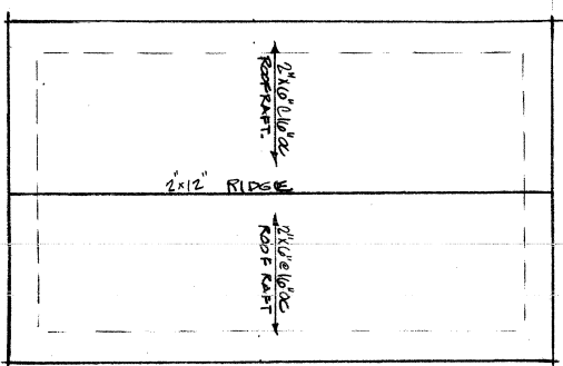
ROOF PLAN SCALE 1/4"=1'-0"
