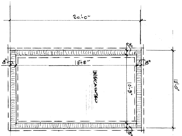
FOUNDATION PLAN SCALE 1/4"=1'-0"
