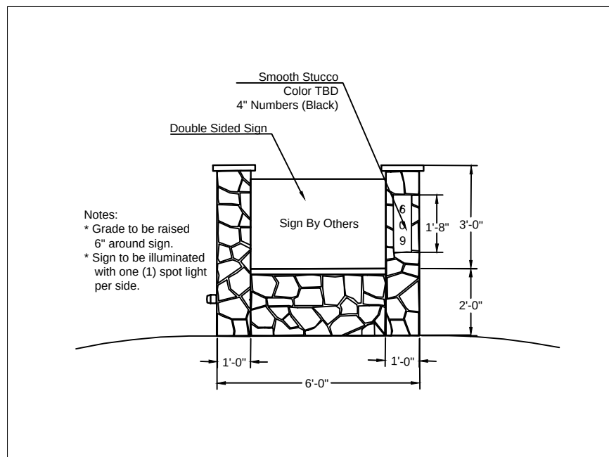
Monument Sign Elevation Scale: 1/4" = 1'=0"
