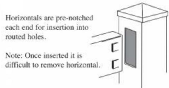
Post/Rail Detail
