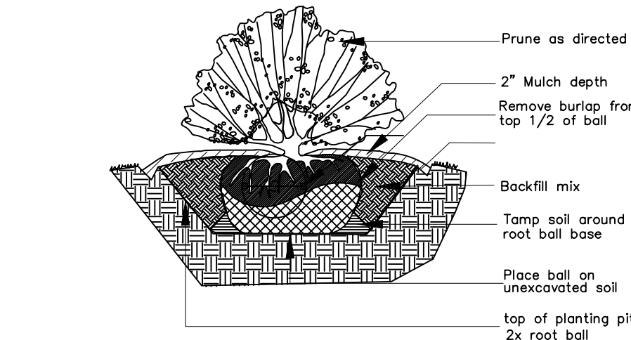
Typical Shrub Planting Detail Not to Scale
