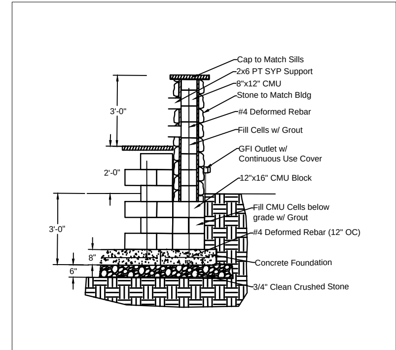
Monument Sign Section Scale: 1/4" = 1'=0"
