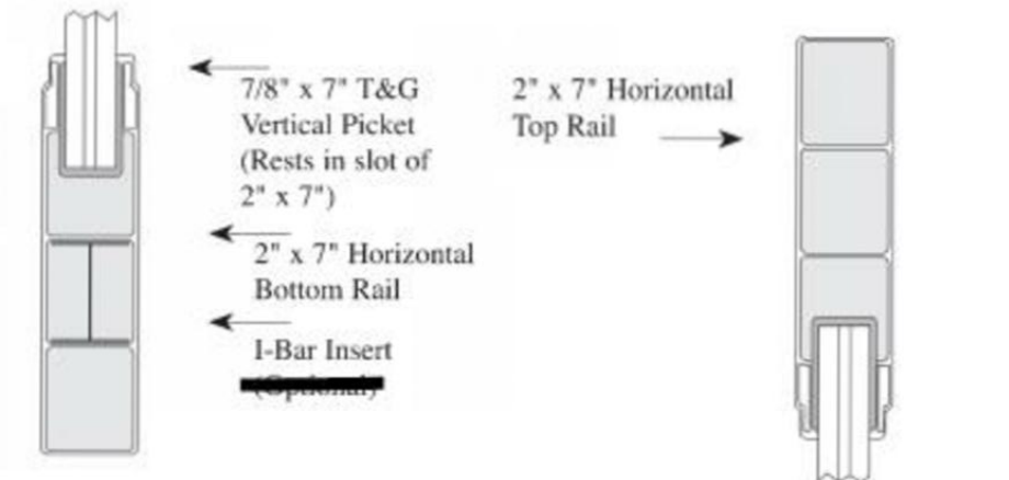
Bottom Rail Detail
