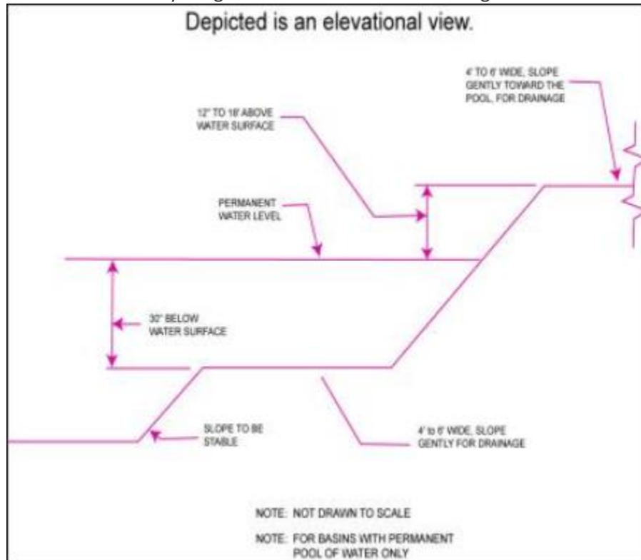
Illustration of Safety Ledges in a New Stormwater Management Basin.
