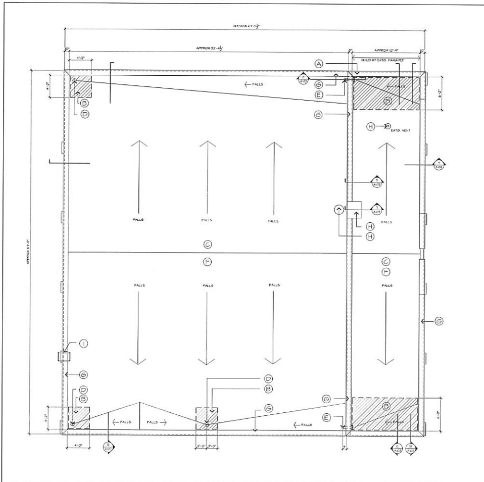
ROOF PLAN
